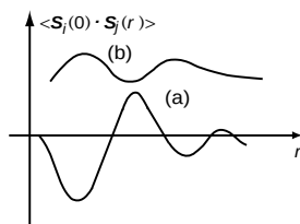
Averaged spin correlations in (a) a speromagnet and (b) an asperomagnet.
