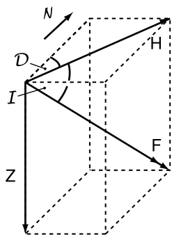
Horizontal and vertical components H , Z of the Earth's field, which has magnitude F , and direction defined by the declination (variation) D and inclination (dip) I .
