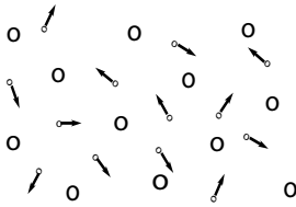
The Born-Oppenheimer approximation: the electrons (marked with arrows) move in a background of frozen nuclei (open circles).
