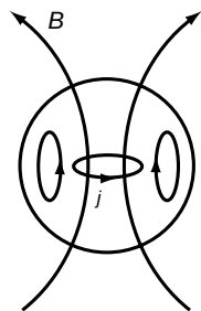
Poloidal field
