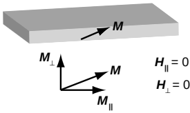
Neither component of a uniformly magnetized thin film produces a stray field.
