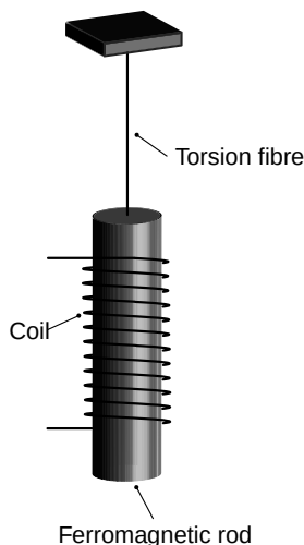
The Einstein-de Haas effect, demonstrating the relation between angular momentum and magnetic moment. A ferromagnetic rod is suspended on a fibre and the field in the solenoid is reversed, switching the direction of magnetization; the rod turns.
