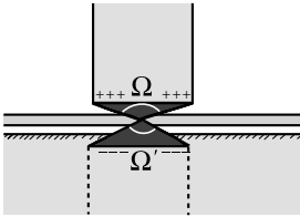
The solid angle subtended by the medium at the write pole and its image.
