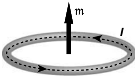
A magnetic moment \mathbf{m} is equivalent to a current loop.
