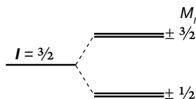
Quadrupole splitting of the energy levels of a nucleus with I = \frac{3}{2} .
