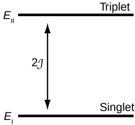
Splitting of the spin singlet and spin triplet states for the \text{H}_2 molecule. The exchange integral \mathcal{J} is negative, so the singlet is lower.
