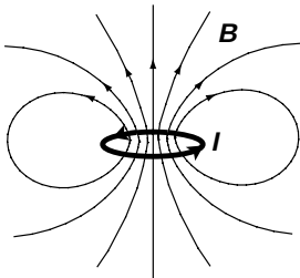
Field due to a current loop.
