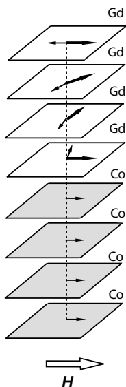
A field-controllable domain wall in an \text{YCo}_2 - \text{GdCo}_2 bilayer.
