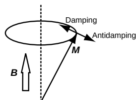
Precession of magnetization with antidamping due to spin-transfer torque.
