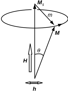
Magnetization precession.
