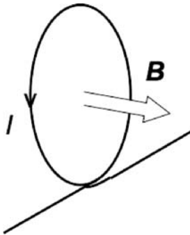
A current loop, with inductance L creates flux \Phi = B \mathcal{A} = L I .
