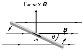
A magnet in a field. The energy is -mB\cos\theta and the torque is mB\sin\theta .
