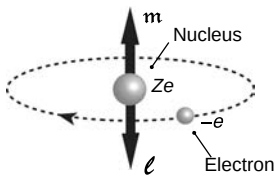
The Bohr atom. The electron moves in a circular orbit where its quantized angular momentum \ell and magnetic moment m are oppositely directed.
