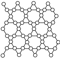
Kagomé lattice
