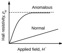
Anomalous Hall effect.
