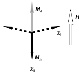
Calculation of the susceptibility of an antiferromagnet well below T_N . The dashed lines show the configuration after a spin flop.
