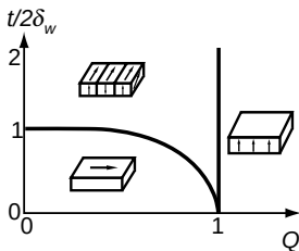
Magnetic domains in a thin film as a function of Q and film thickness t .
