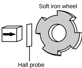
Variable-reluctance sensor based on a permanent magnet.
