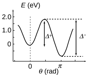
Energy barrier to magnetic reversal of a superparamagnetic particle in an applied field.
