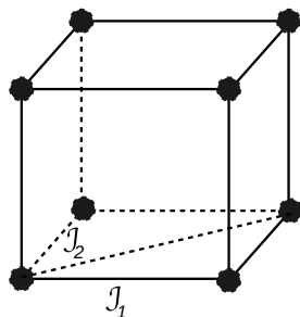
Magnetic interactions in a simple cubic lattice.
