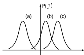
Distributions of exchange interactions giving rise to (a) speromagnetism, (b) asperomagnetism and (c) ferromagnetism.
