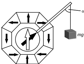
A magnetically compensated hinge.
