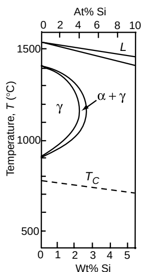
Iron-rich side of the Si-Fe phase diagram.
